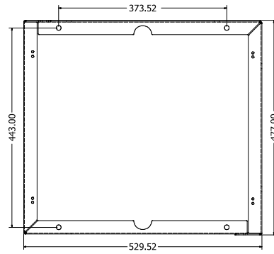
Bracket
