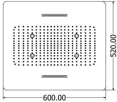
Shower head
